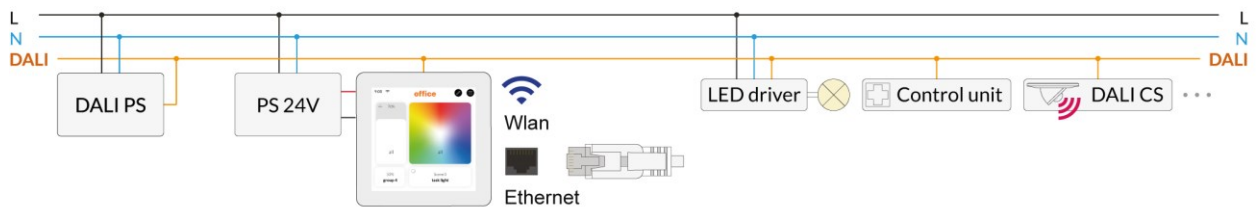
Figure 1 Typical Application
