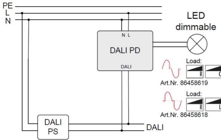
typical structure
